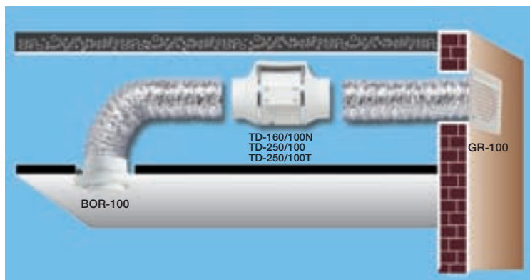
GSA-100 Aluminium flexibel (4m) + alu plakband
